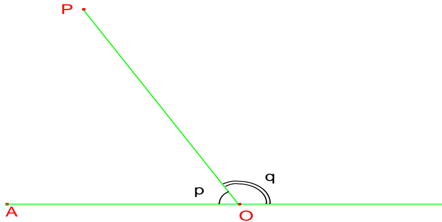
Supplementary Angles
