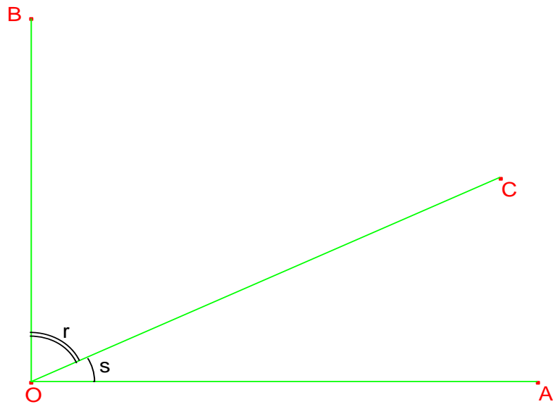
Complementary Angles
